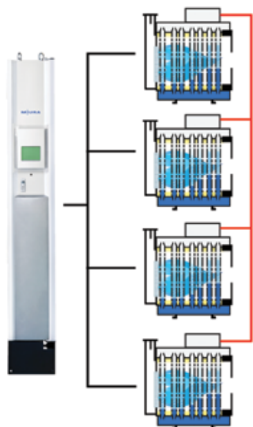
▼ Figure 5. A single automation system can control several modular boilers.
